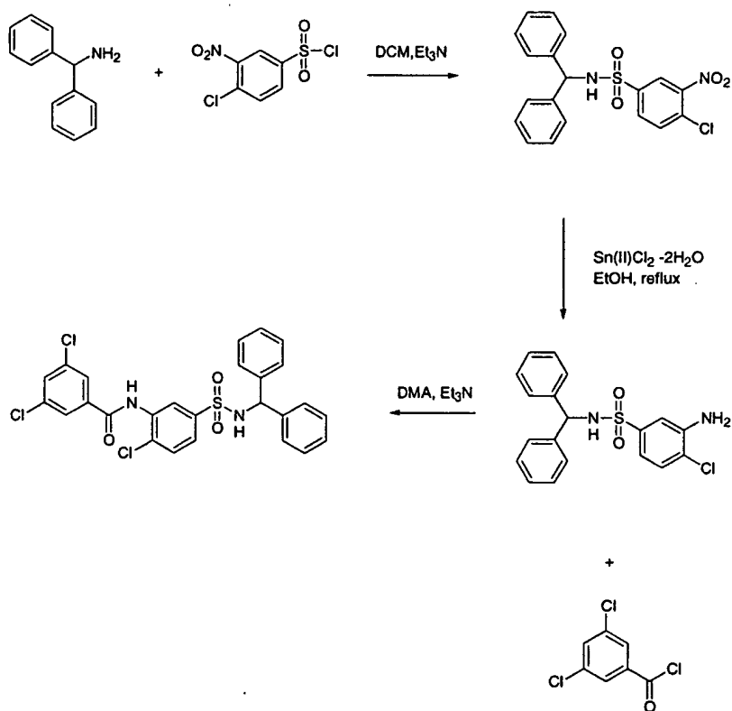
Scheme X
